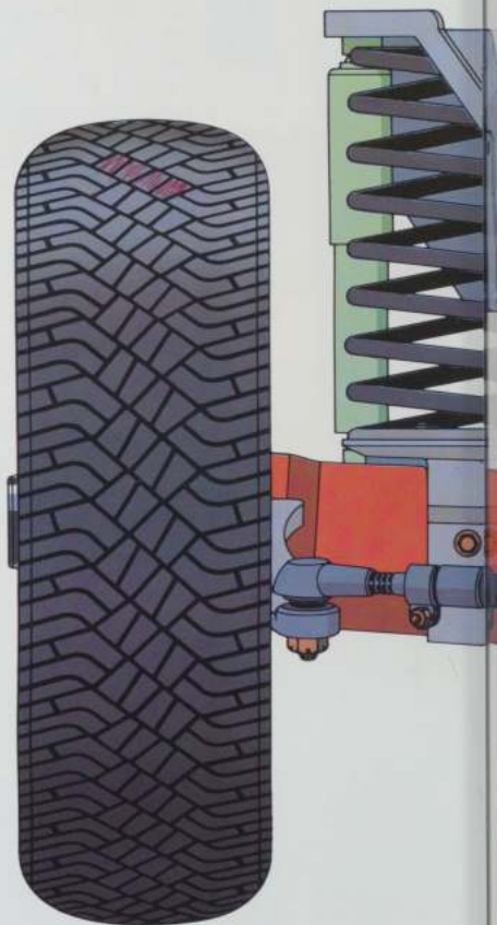
Ford-famous Twin-I-Beam independent front suspension is standard with the 2WD model and the Twin-Traction Beam system (shown above) with the 4WD. Each front wheel, with its own axle and hefty coil spring, steps over bumps independently to help cushion the ride and provide excellent handling.
