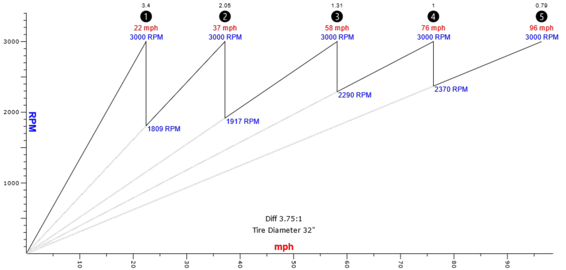
mph - Diff 3.75 - Tire - 32"
