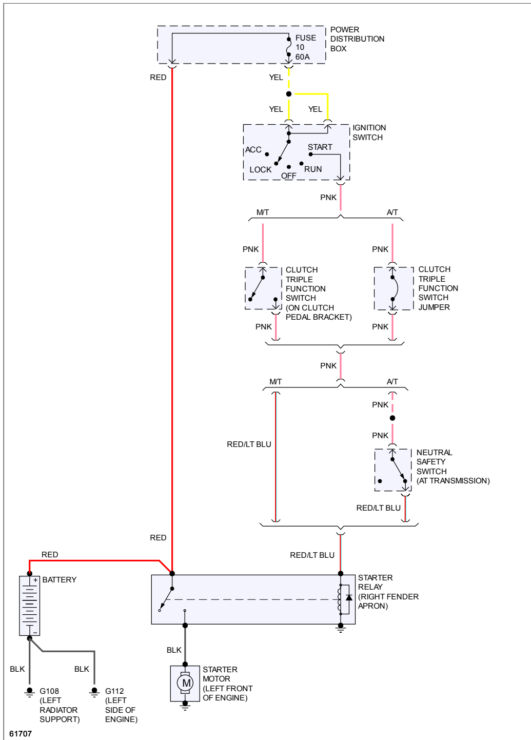
Fig 2: Starting Circuit
